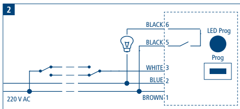
New connection with the 220 V AC powered Domotic RX with 1 output
