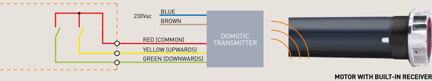
MOTOR WITH BUILT-IN RECEIVER
