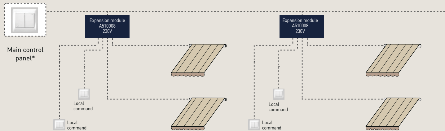
MOTOR WITH WIRE CONTROL
